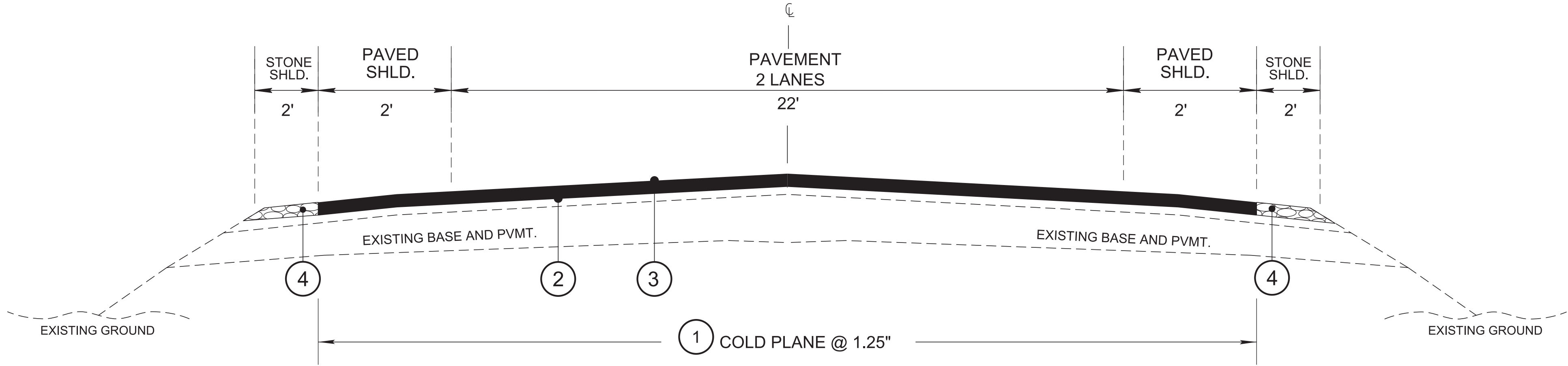
SR-13 TYPICAL SECTION L.M. 31.5 TO L.M. 38.45
